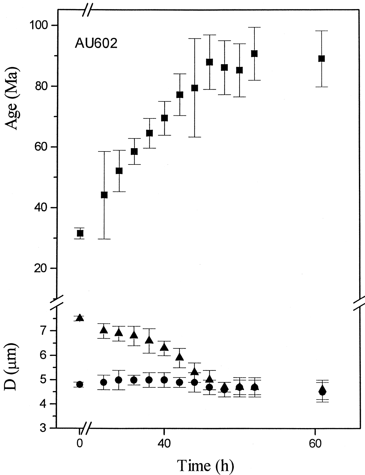
Figure 1. Plateau age for Australian obsidian AU602 obtained by using isothermal treatment (upper represented by squares). Induced (pyramids) and spontaneous (circles) fission-track diameters at each step of thermal treatment (lower).
